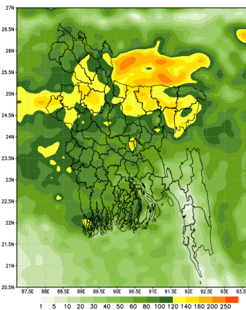
Simulated Rainfall (mm) (WRF model) Period (01-05-2020 to 09-05-2020)
